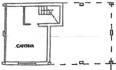
PIANO SEMINTERRATO H=240
